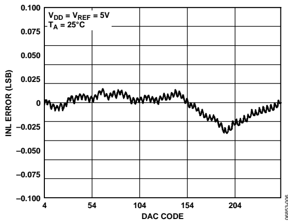
Figure 7. Typical AD5601 INL
