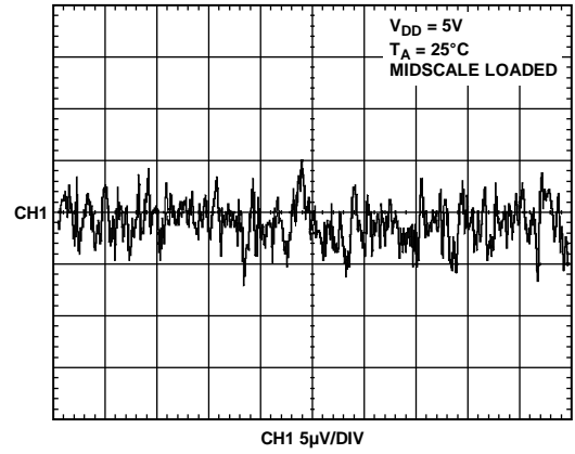
Figure 20. 1/f Noise, 0.1 Hz to 10 Hz Bandwidth
