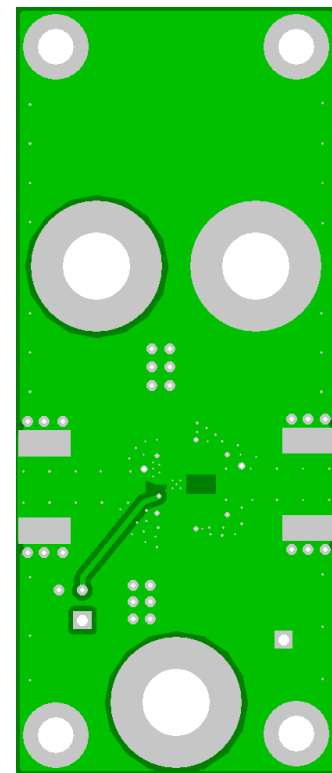
Figure 55. THS4302EVM Board Layout (Bottom Layer)
